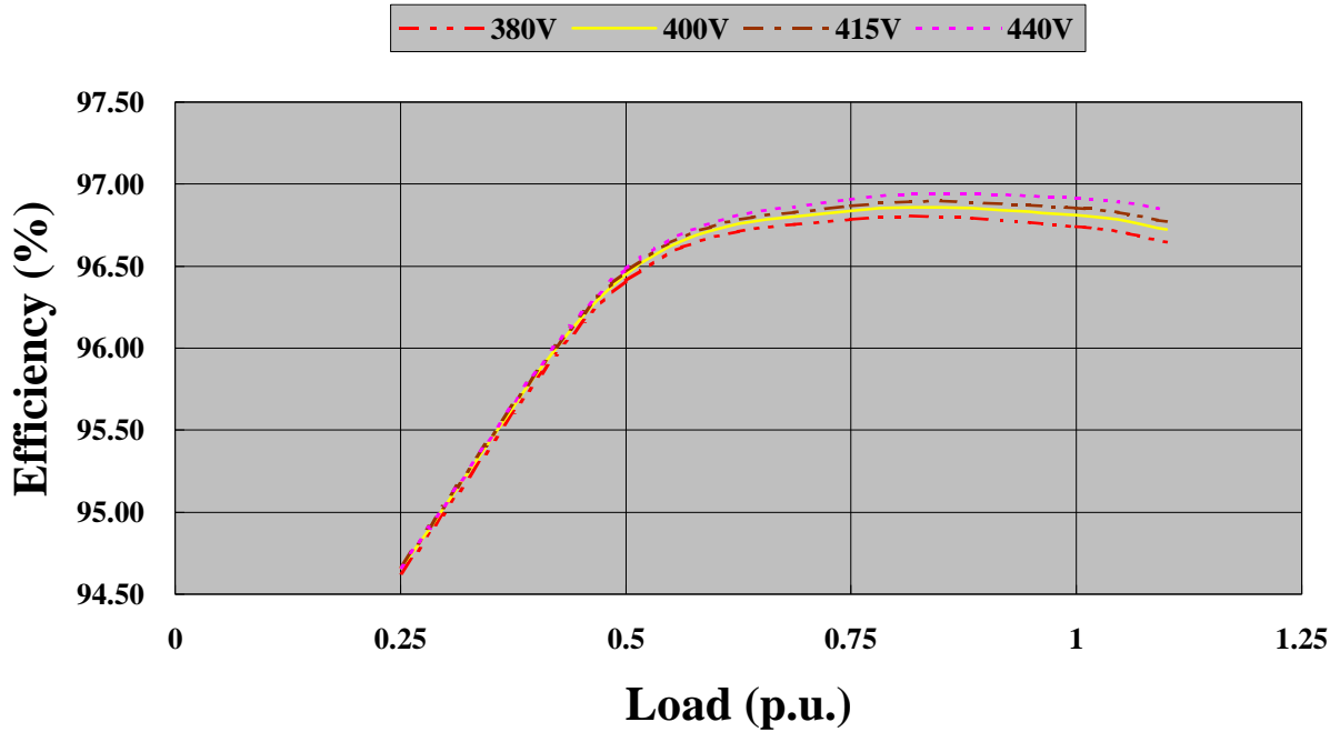
EG500-1920N - 50Hz at 1500rpm PF 1
