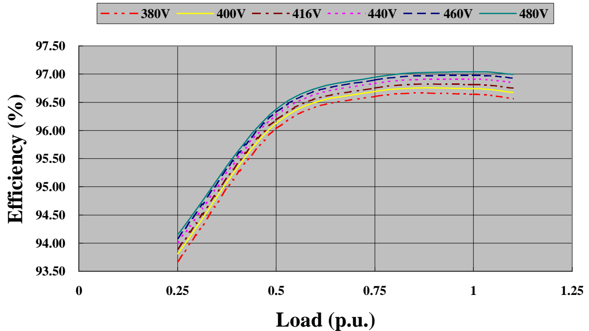
EG500-1920N - 60Hz at 1800rpm PF 1
