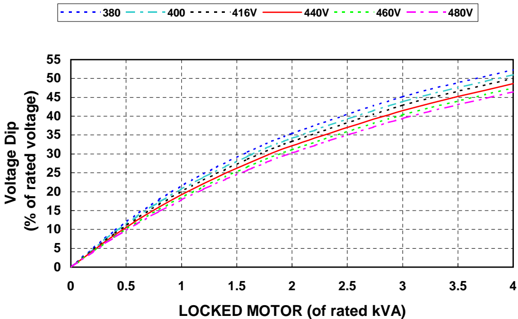
LOCKED ROTOR MOTOR STRATING CURVES AT 60Hz
