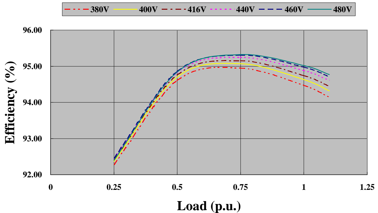
EG400-720N - 60Hz at 1800rpm PF 0.8
