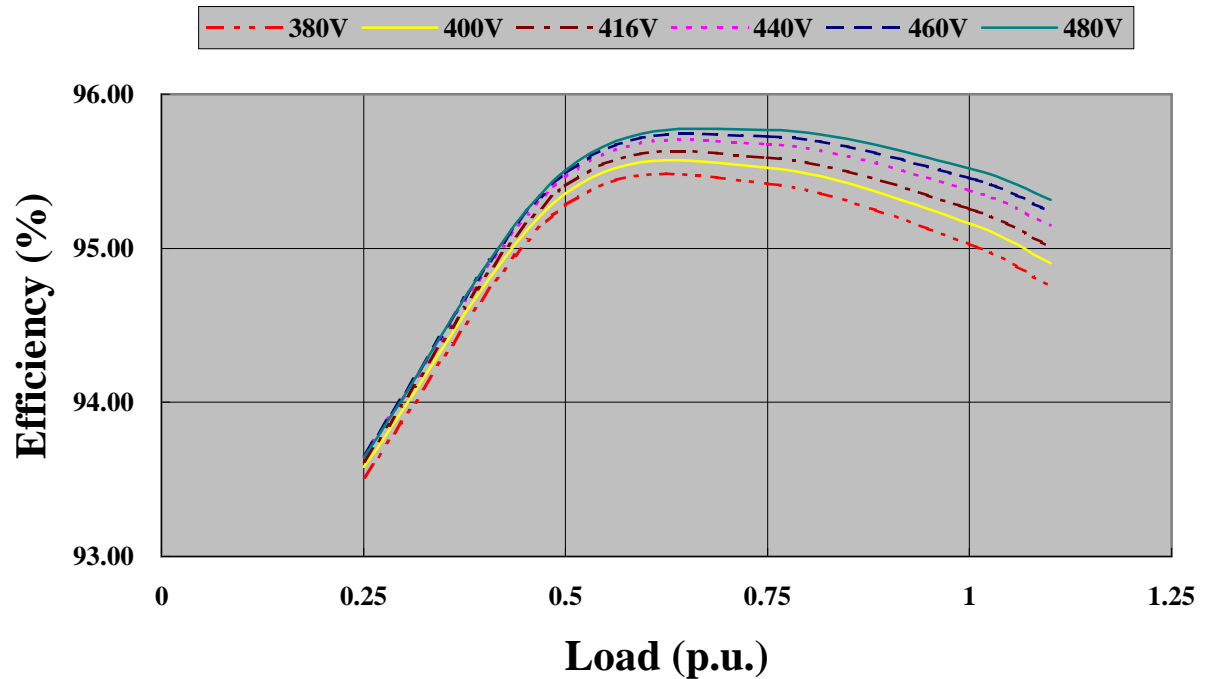
EG400-1000N - 60Hz at 1800rpm PF 0.8
