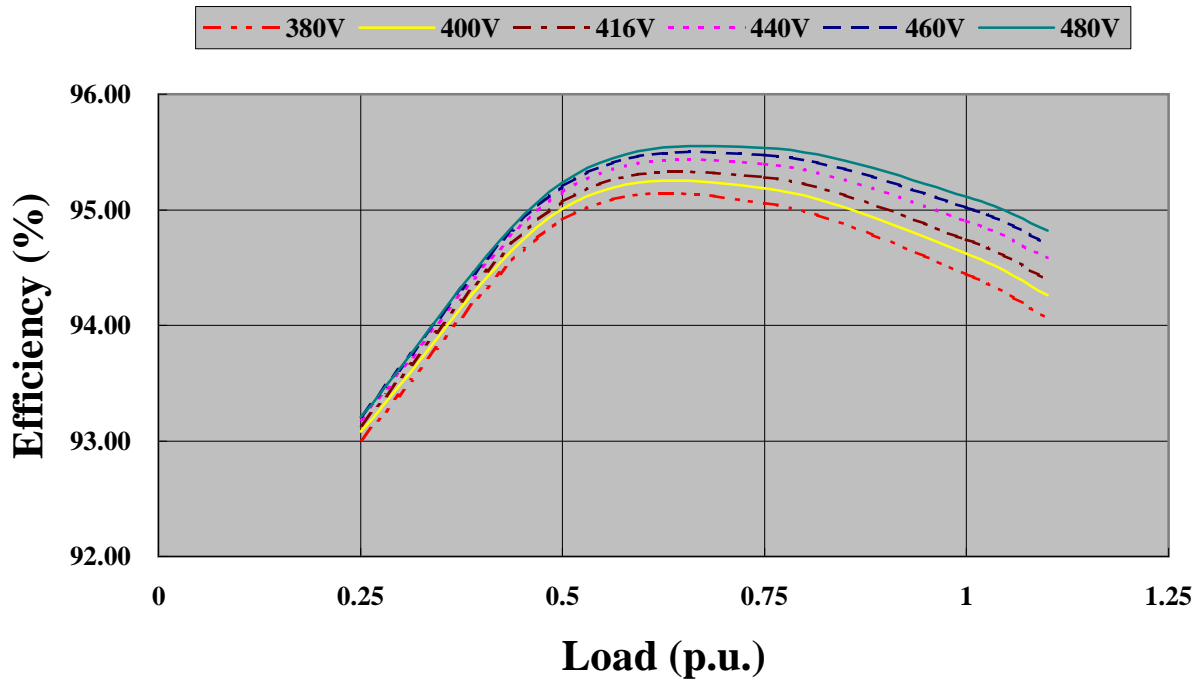
EG355-560N - 60Hz at 1800rpm PF 0.8
