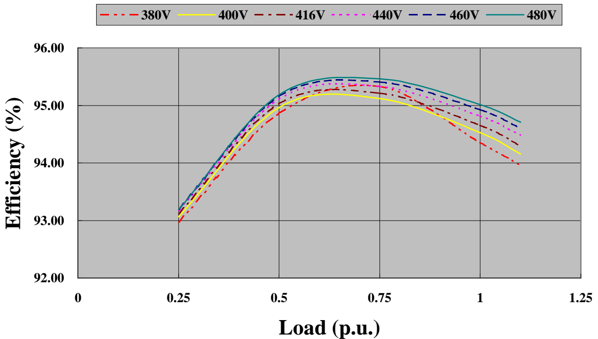
EG355-500N - 60Hz at 1800rpm PF 0.8
