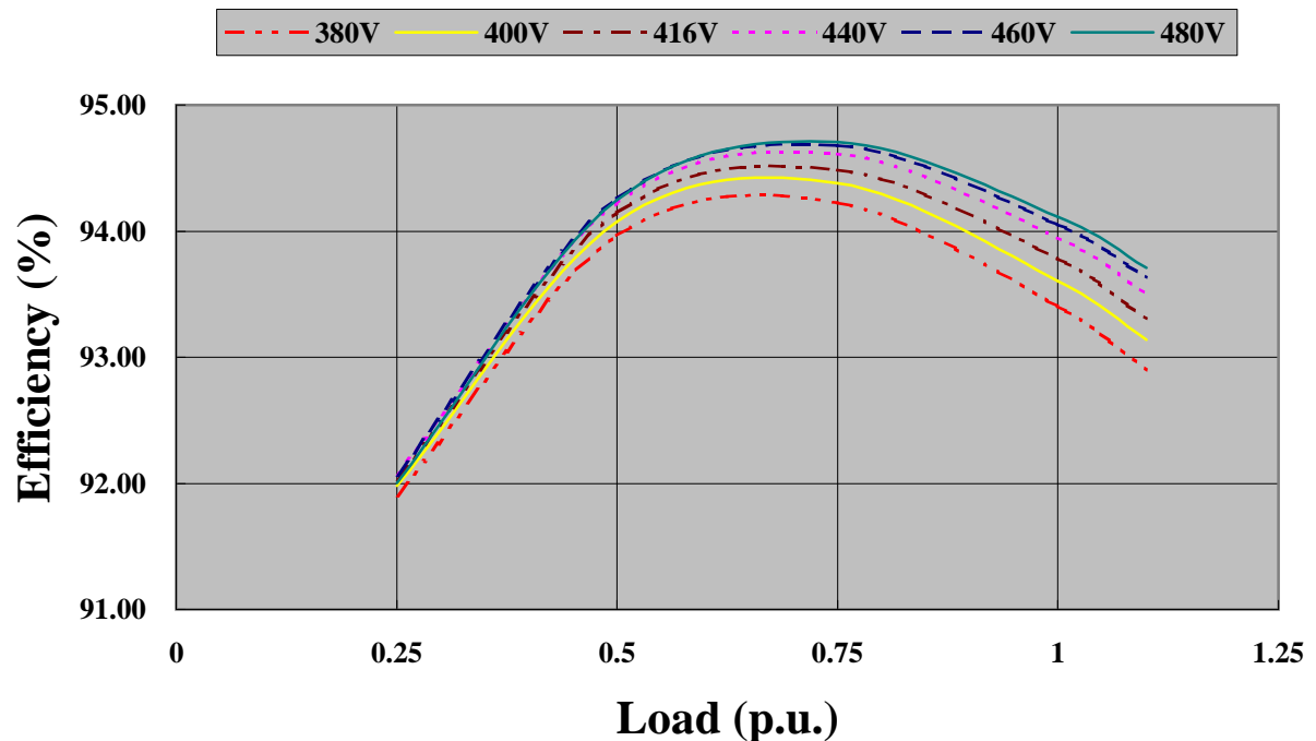
EG315-300N - 60Hz at 1800rpm PF 0.8
