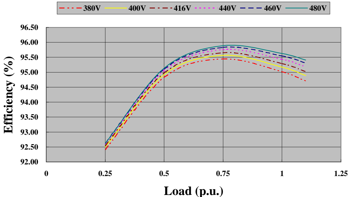
EG315-280N - 60Hz at 1800rpm PF 1
