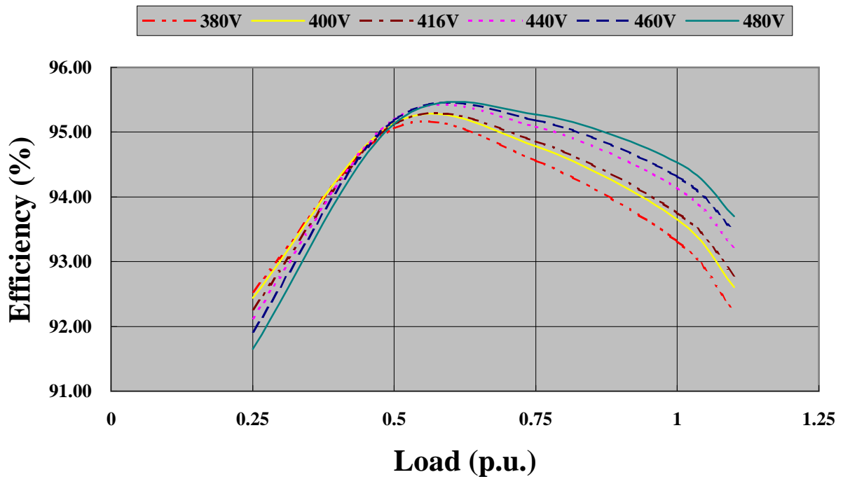
EG225-90N - 60Hz at 1800rpm PF 1
