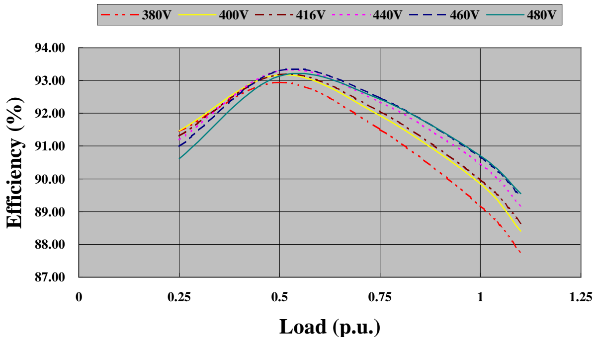
EG225-90N - 60Hz at 1800rpm PF 0.8
