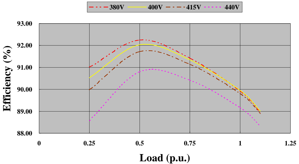
EG225-90N - 50Hz at 1500rpm PF 0.8
