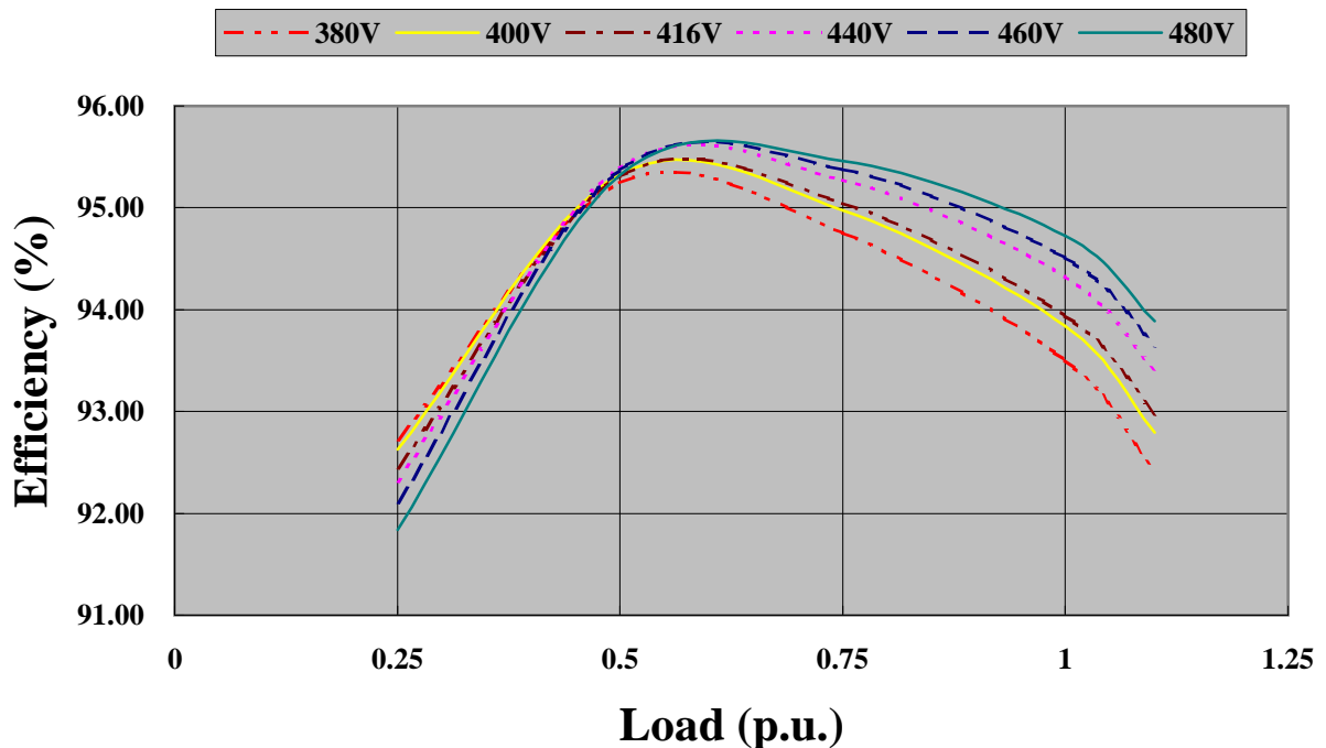
EG225-80N - 60Hz at 1800rpm PF 1
