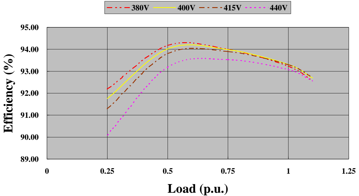
EG225-80N- 50Hz at 1500rpm PF 1
