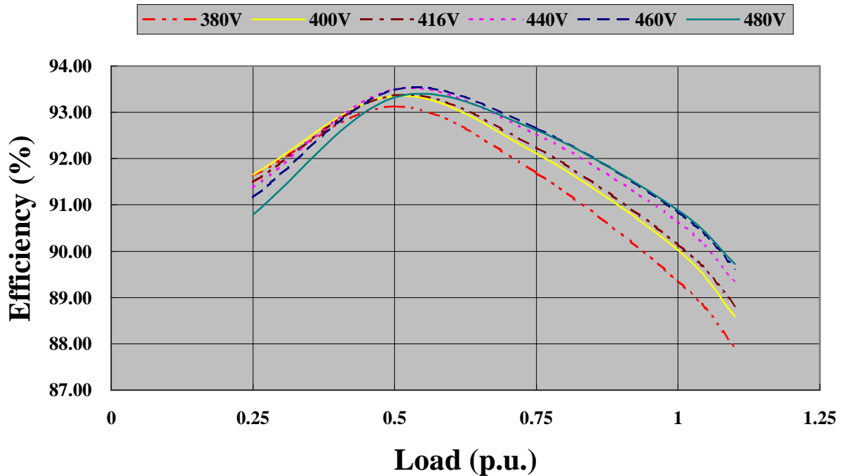
EG225-80N - 60Hz at 1800rpm PF 0.8
