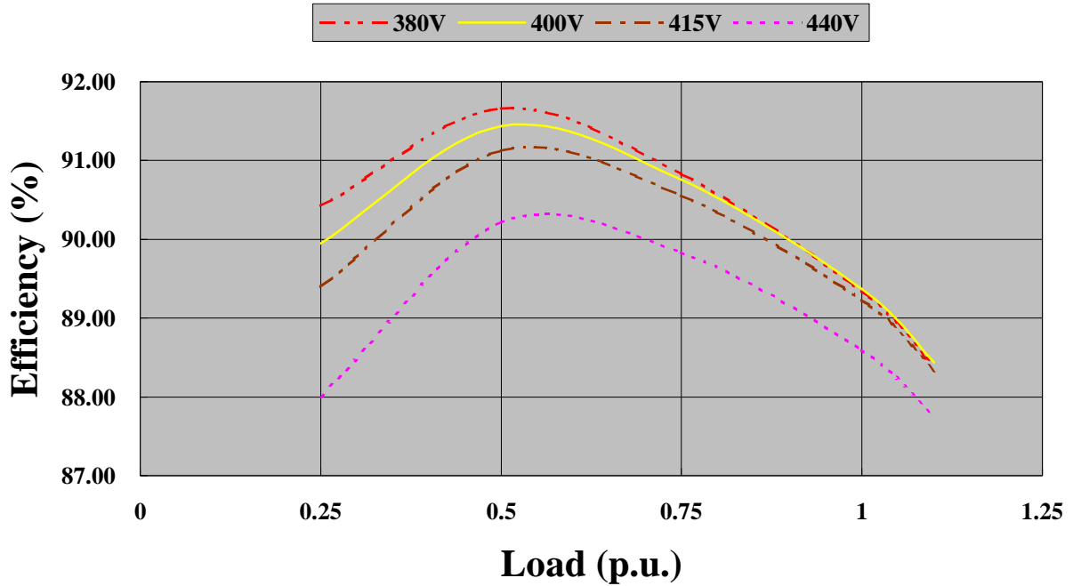
EG225-70N - 50Hz at 1500rpm PF 0.8
