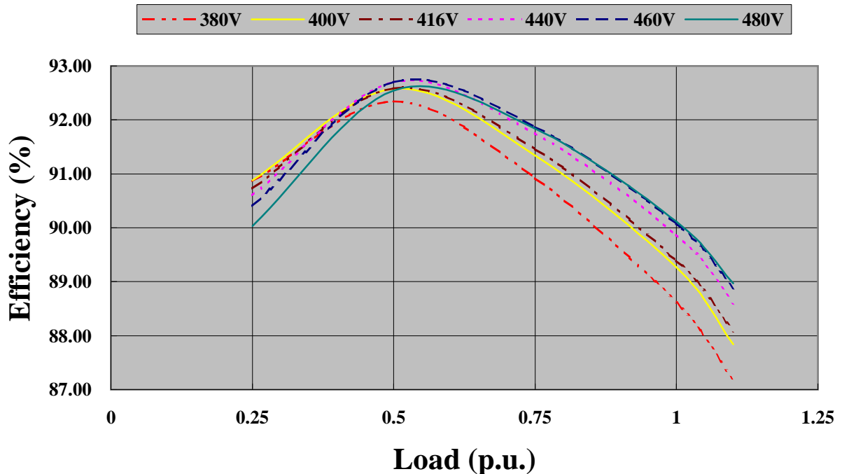
EG225-70N - 60Hz at 1800rpm PF 0.8
