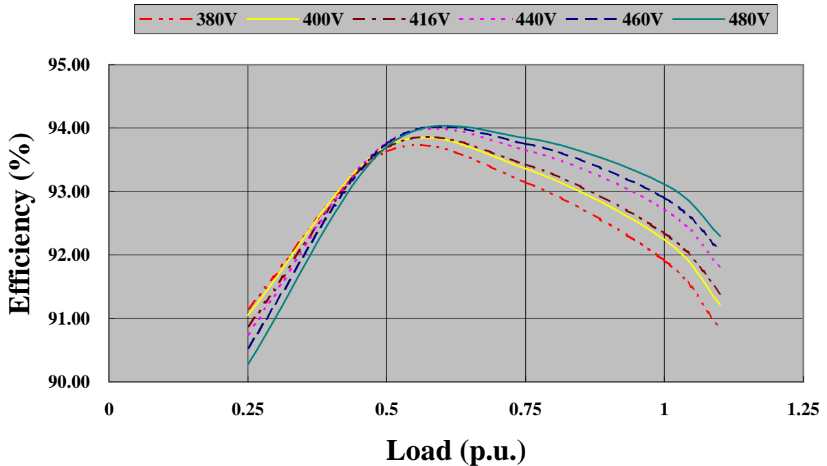
EG225-60N - 60Hz at 1800rpm PF 1
