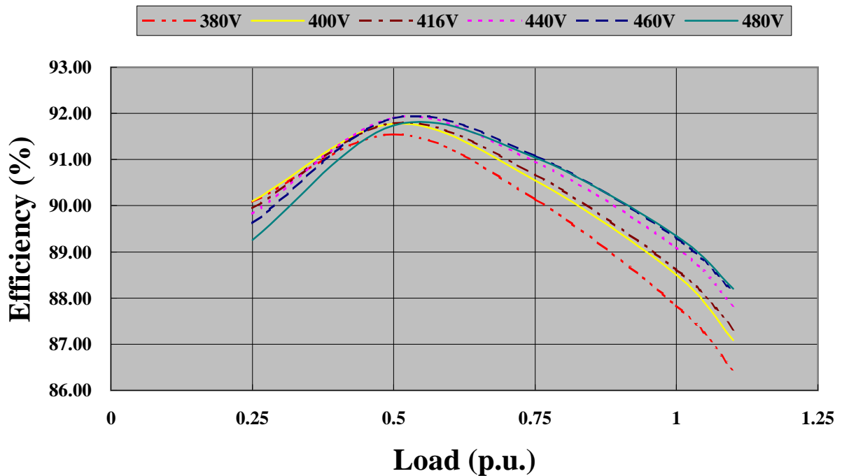
EG225-60N - 60Hz at 1800rpm PF 0.8
