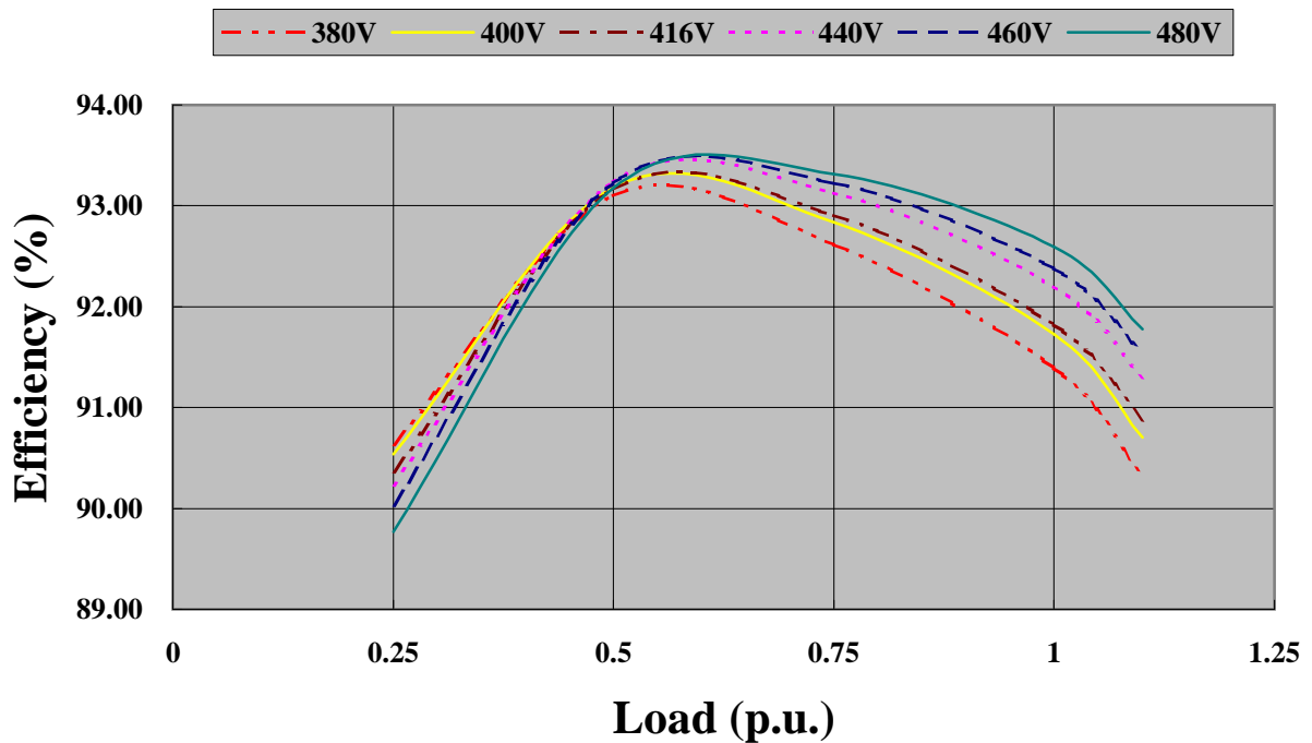
EG225-50N - 60Hz at 1800rpm PF 1
