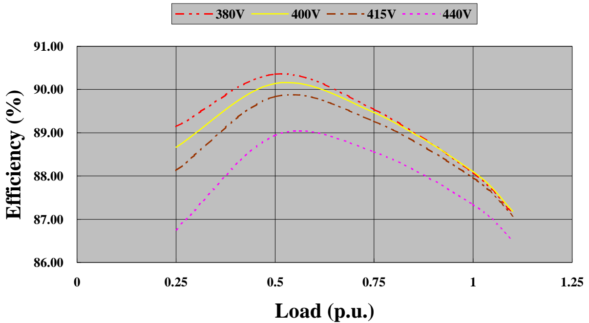
EG225-50N- 50Hz at 1500rpm PF 0.8
