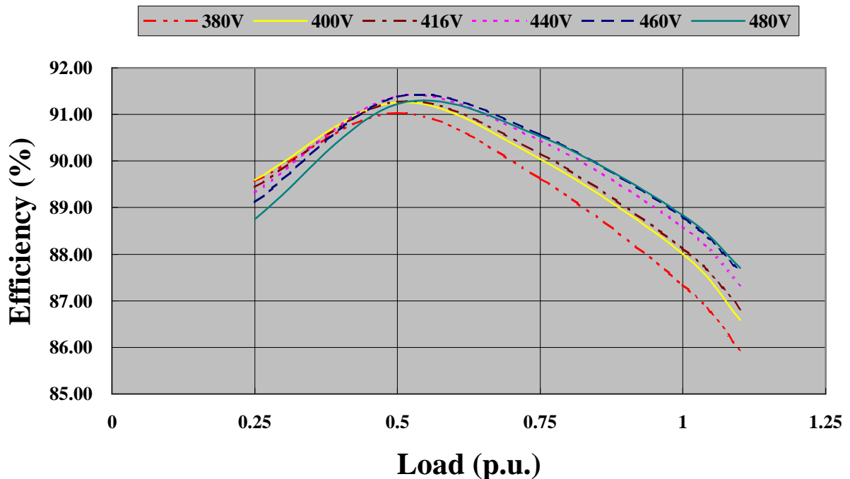
EG225-50N - 60Hz at 1800rpm PF 0.8
