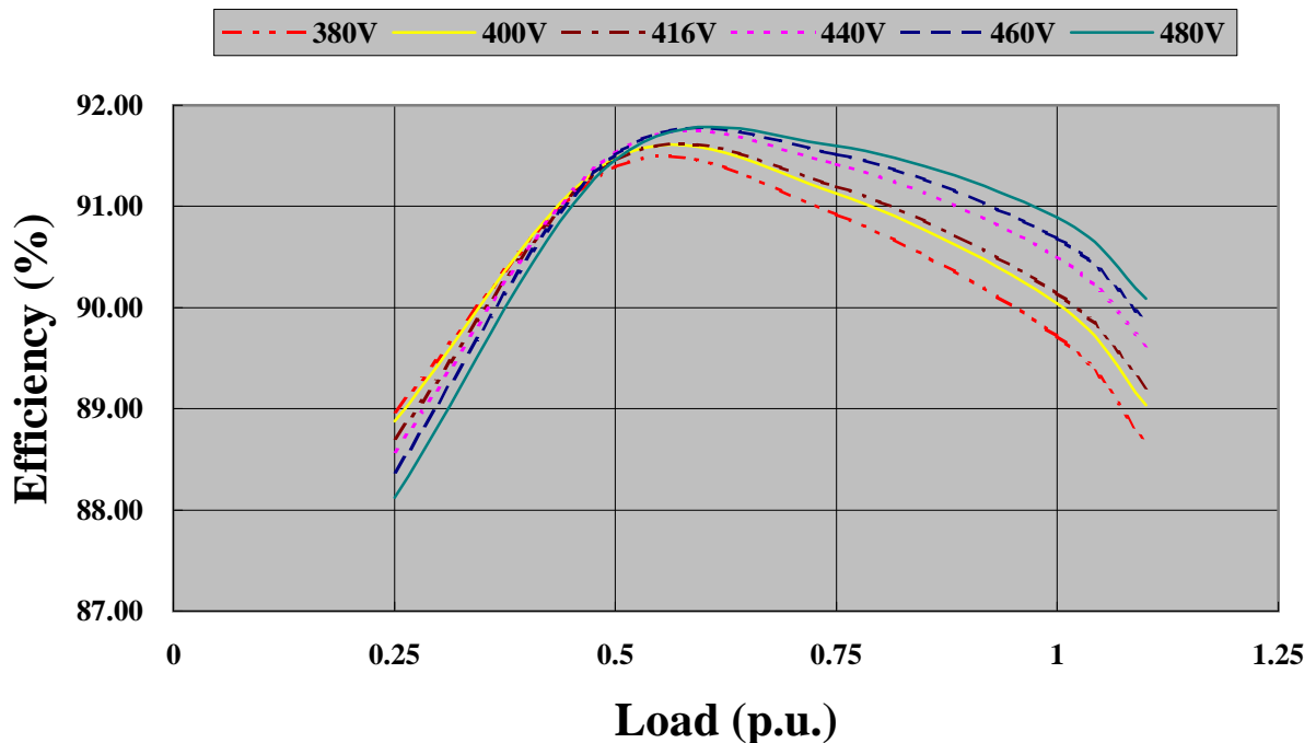
EG225-40N - 60Hz at 1800rpm PF 1
