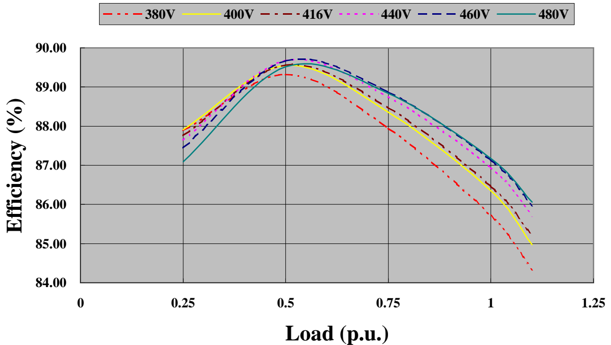
EG225-40N - 60Hz at 1800rpm PF 0.8
