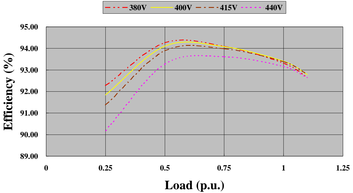
EG225-100N- 50Hz at 1500rpm PF 1
