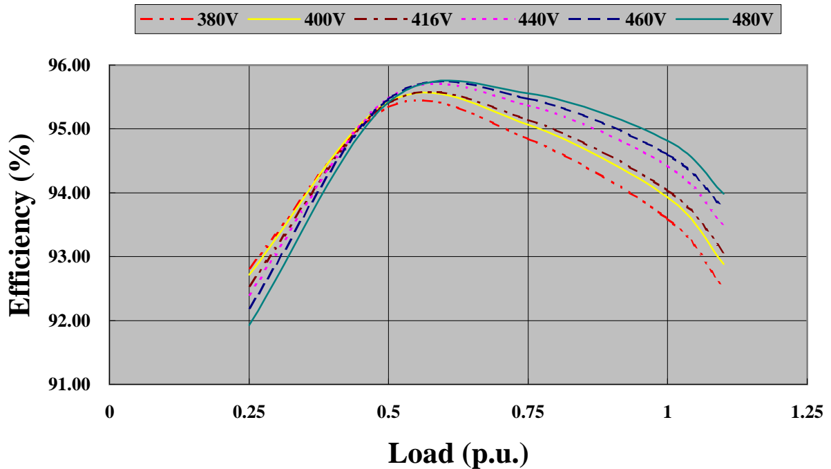
EG225-100N - 60Hz at 1800rpm PF 1
